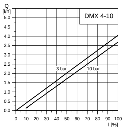
DMX 4-10
