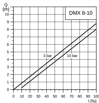
DMX 8-10
