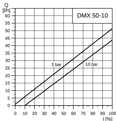
DMX 50-10
