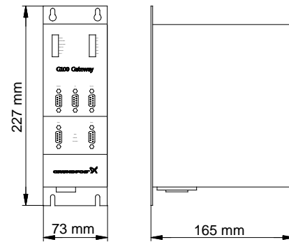
Fig. 18 Dimensional sketch
