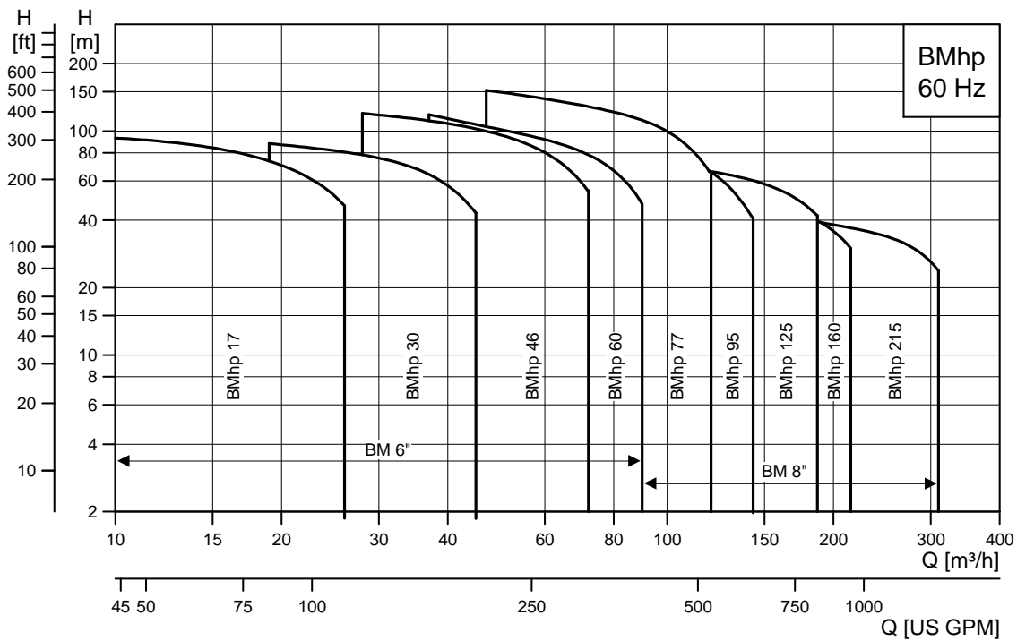
Fig. 4 Performance range, BMhp 60 Hz
